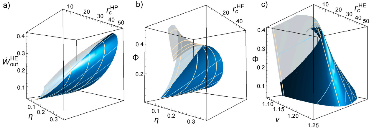
Fig. 6. Behaviors of power output \dot{W}_{out}^{HE} versus \eta , \Phi versus \eta and \Phi versus v in terms of the compression ratios r_c^{HE} by the parametric elimination of r_c^{HP} . The baseline arrangement is as in previous figure.
