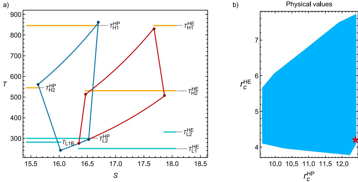
Fig. 11. Argon-solar salt-methanol system: T-S cycle (blue is the charge process and red the discharge one) and physically suitable values of the r_c^{HP} and r_c^{HE} values (blue surface); the red star denotes the values of these parameters for the particular depicted configuration. \epsilon_c = \epsilon_r = 0.9 , \epsilon_H = 0.95 , \epsilon_L = 0.9 , \Delta P = 0.01 , \xi = 0.02 , \gamma = 1.667 , \Gamma_H^{HE} = \Gamma_H^{HP} = 1 , \Gamma_L^{HE} = \Gamma_L^{HP} = 0.35 , PP_H = 10 K, PP_L = 4 K. Values for the simulation: T_{max} = 858 K and T_{min} = 511 K are the maximum and minimum values of the salt temperature; T_{L,max} = 351 K and T_{L,min} = 175 K for the maximum and minimum values of the liquid methanol temperature; and initial value of the T_{H2}^{HP} = 550 K, r_c^{HP} = 12.4 and r_c^{HE} = 4.2 .
