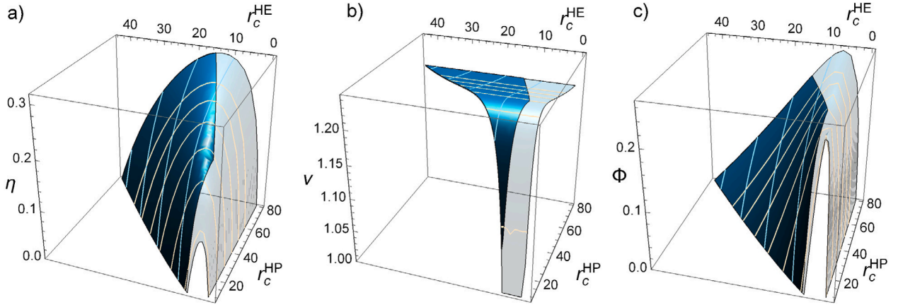
Fig. 5. Behaviors of \eta , v and \Phi in terms of the compression ratios r_c^{HE} and r_c^{HP} . Baseline arrangement: \epsilon_c = \epsilon_l = 0.9 , \epsilon_H = \epsilon_L = 0.90 , \Delta P = 0.02 , \xi = 0.02 , T_{H2}^{HP} = 500 K, T_{L2}^{HP} = T_0 = 300 K, T_{L1}^{HE} = 250 K, \gamma = 1.4 , \Gamma_H^{HE} = 1 , \Gamma_L^{HE} = 0.4 , \Gamma_H^{HP} = 0.9 , \Gamma_L^{HP} = 1 , PP_H = PP_L = 0 K. The transparent surfaces contains values without any constraint on the input parameters.
