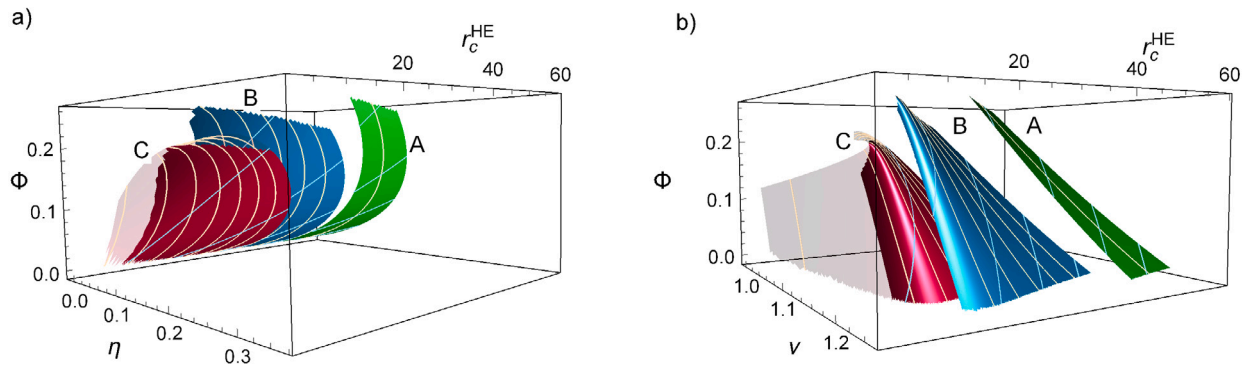
Fig. 10. Effects of the external irreversibilities on the parametric plots of \Phi , \eta and \nu versus r_c^{HE} with PP_H = PP_L = 5 . The legend and numerical values of parameters are the same that in Fig. 8.
